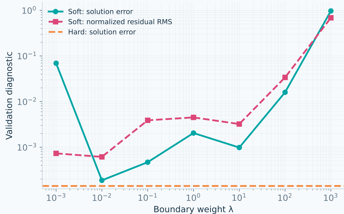
A larger penalty need not help accuracy
